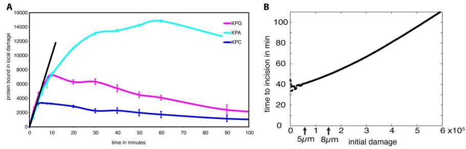
Figure S4. NER rate. (A) Cells expressing XPC-EGFP, XPG-EGFP, and EGFP-XPA were locally irradiated (5- \mu\text{m} pores; 100 J.m -2 ) as described in Materials and methods. The binding curve shows the first 100 min of the binding curve shown in Fig. 2 B. The assembly rates of these NER proteins can be estimated from the initial slope of the binding curves. The tangent shows an immobilization of \sim 3.6\% , \sim 1.1\% , and \sim 0.5\% of the total protein pool per minute for XPC, XPG, and XPA, respectively. Given that the concentrations of XPC (about three 10^4 molecules/cell), XPG (about eight 10^4 molecules/cell), and XPA (about two 10^5 molecules/cell) are different (Araújo et al., 2001), this tangent translates to assembly rates of \sim 900 molecules/min or \sim 15 molecules/s for XPC, XPG, and XPA. (B) Computation of the mean time to incision in the model versus the initial amount of DNA damage (6-4 PPs). The arrows indicate the amounts of damage estimated for the experimental setup with UV-permeable pores of 5- and 8- \mu\text{m} diameter.
