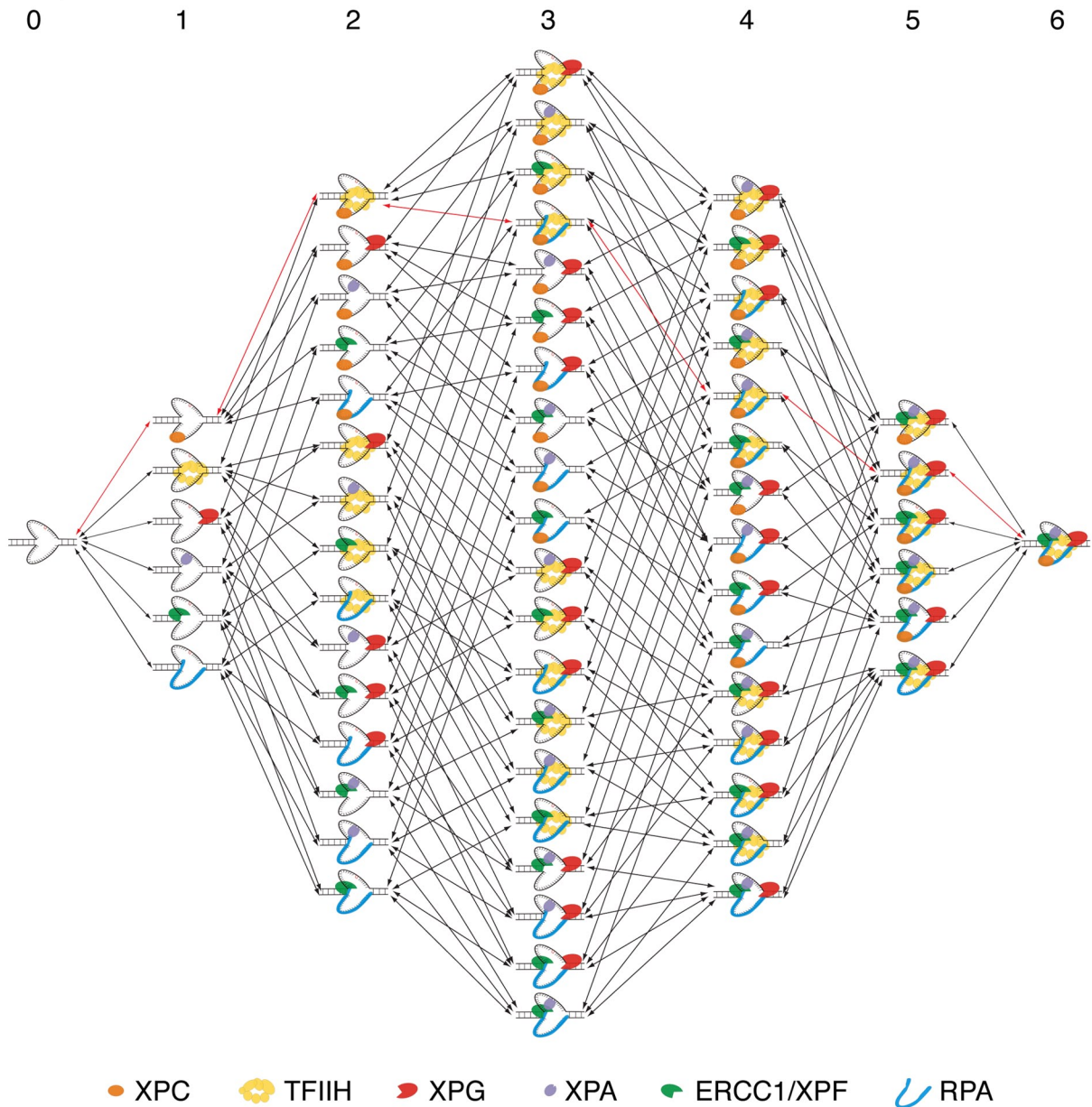
Figure 5. Kinetic model of NER. The model distinguishes six DNA repair intermediates, as indicated, that are interconverted by enzymatic steps. Red arrows: \alpha , partial DNA unwinding; \alpha' , full unwinding; \beta , dual incision; \gamma , resynthesis; \delta , rechromatinization; \epsilon_1 and \epsilon_2 , reannealing of unwound DNA when it becomes devoid of stabilizing proteins. The indicated NER proteins can bind to the repair intermediates. The binding of TFIIH to the DNA lesion requires the prior binding of XPC. The binding of XPA and ERCC1/XPF is cooperative (Table S1). (B) Possible assembly pathways for the preincision complex on unwound DNA. Random assembly can use all pathways shown, whereas sequential assembly will follow a unique pathway (e.g., the pathway indicated by the red arrows assuming ordered binding of XPC, TFIIH, RPA, XPA, XPG, and ERCC1/XPF).
