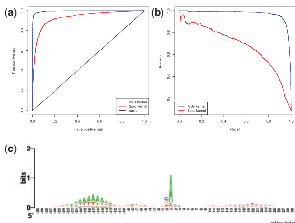
Fig. 4. (a) ROC curve for the classification of WD kernel and Spectrum kernel on constitutive PAS clusters versus background. WD outperformed the Spectrum kernel (auROC = 99.6, 93.5%). (b) PRC curve. (c) Sequence Logo for (-30,+30) region around PAS clusters for constitutive genes; PAS site at position 0
