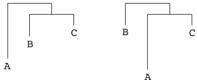
Figure 2. Sampling of Tree Topologies
