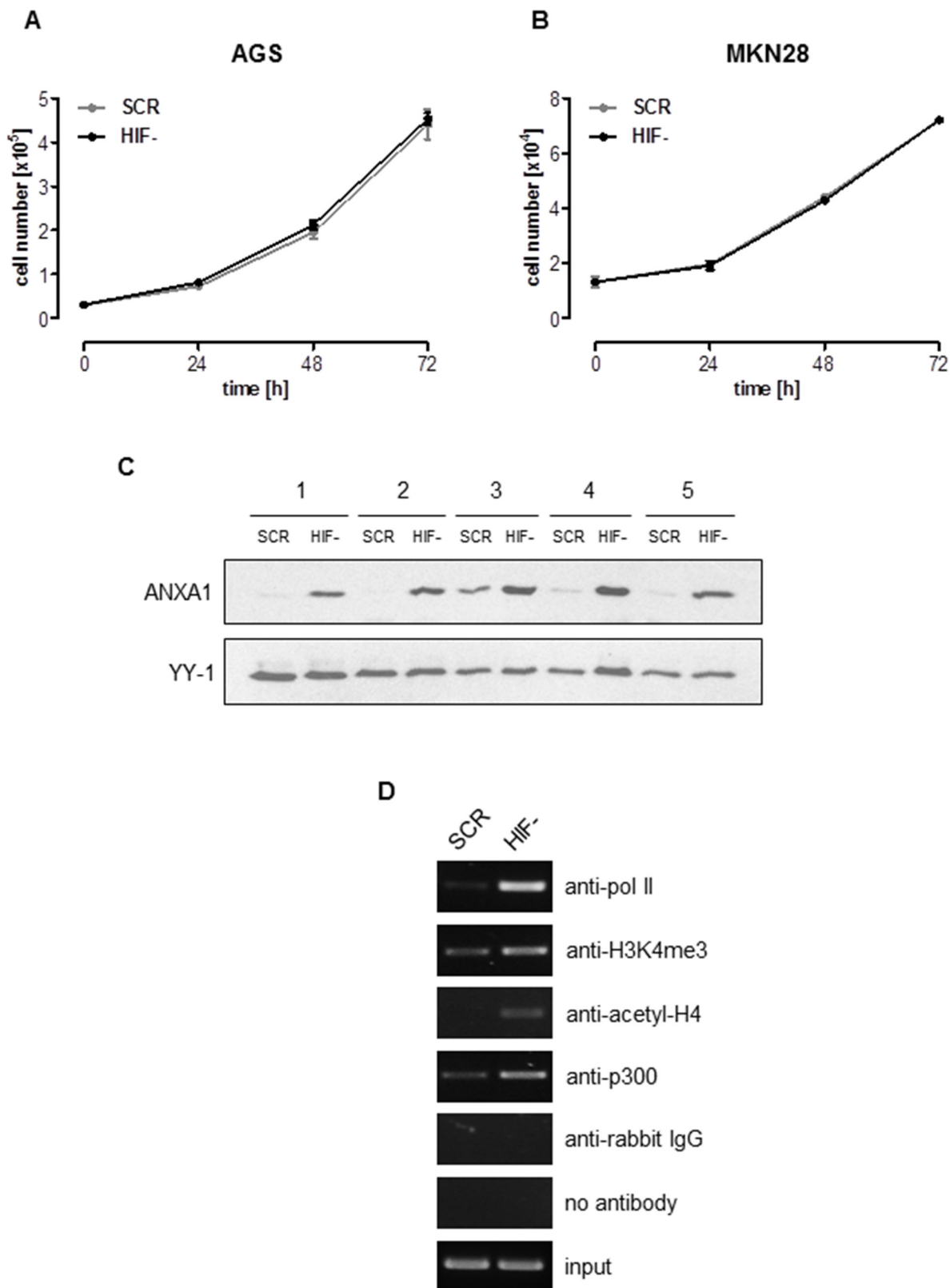
Figure 1: ANXA1 is a crucial mediator of HIF-1 \alpha -independent cellular proliferation. (A, B) Anchorage-dependent proliferation of HIF-1 \alpha -deficient (HIF-) and control (SCR) AGS and MKN28 cells under normoxia. Results shown are representative of three independent experiments and values represent the mean \pm SEM of triplicate determinations. (C) Analysis of ANXA1 expression in AGS HIF- and SCR cells by immunoblot using whole cell lysates harvested at five different time points. YY-1 served as loading control. (D) Chromatin status of the ANXA1 promoter in AGS HIF- and SCR cells was determined by chromatin immunoprecipitation. Representative gels of four independent experiments are shown.
