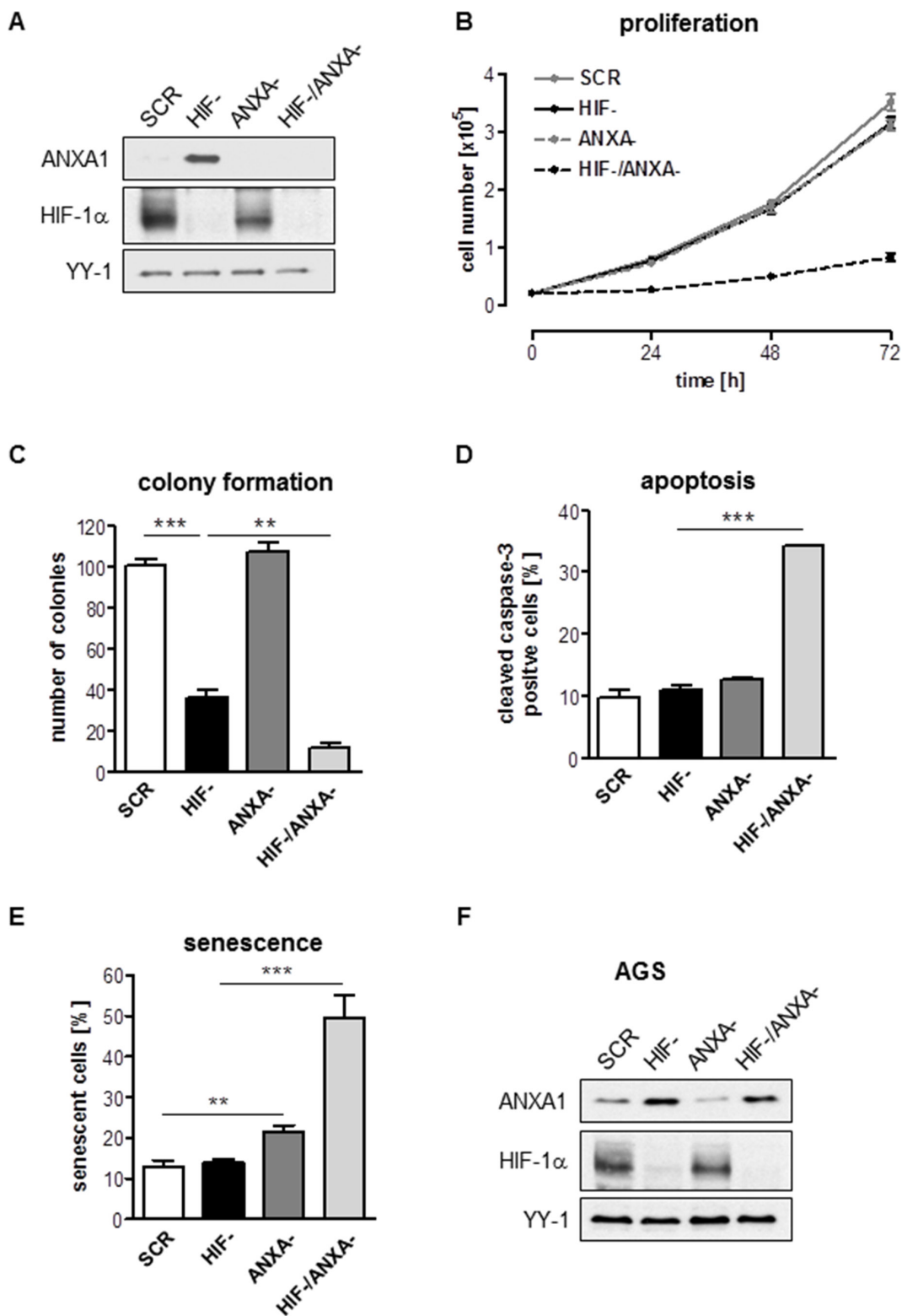
Figure 2: Effects of combined inhibition of HIF-1 \alpha and ANXA1 on AGS cell proliferation. (A) Representative immunoblot analysis of ANXA1 and HIF-1 \alpha in control (SCR), HIF-1 \alpha -deficient (HIF-), ANXA1-deficient (ANXA-) and double knock-down (HIF-/ANXA-) cells. YY-1 served as loading control. (B, C) Anchorage-dependent (B) and anchorage-independent (C) proliferation. Results shown are representative of three independent experiments and values represent the mean \pm SEM of triplicate determinations (** P < 0.01 ; *** P < 0.001 ). (D) Apoptosis was assayed by cleavage of caspase-3 followed by FACS analysis. Values are means \pm SEM (*** P < 0.001 ). (E) Senescence was quantified 96 h after cultivation by measurement of SA- \beta -Gal activity. Values are means \pm SEM (** P < 0.01 ; *** P < 0.001 ). (F) Representative immunoblot analysis of ANXA1 and HIF-1 \alpha . Cells were passaged regularly and grown as monolayer cultures under recommended culture conditions for four weeks. YY-1 served as loading control.
