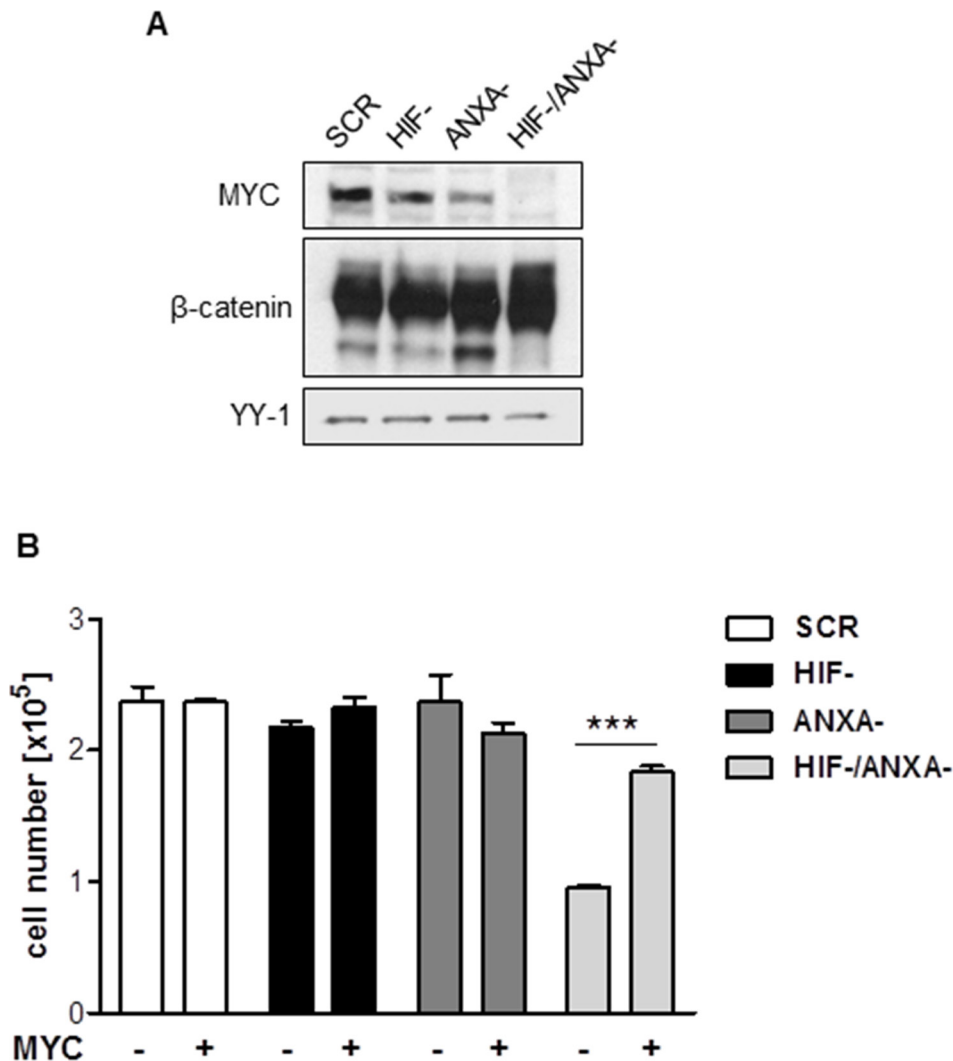
Figure 6: Contribution of MYC to the growth defect in HIF-1 \alpha /ANXA1-deficient cells. (A) Representative immunoblot analysis of MYC and \beta -catenin in control (SCR), HIF-1 \alpha -deficient (HIF-), ANXA1-deficient (ANXA-) and double knock-down (HIF-/ANXA-) AGS cells. YY-1 served as loading control. (B) Re-expression of MYC was achieved by transduction with retroviruses containing human MYC and anchorage-dependent proliferation was analyzed 14 days post transduction. Results shown are representative of three independent experiments and values represent the mean \pm SEM of triplicate determinations (***) P < 0.001 .
