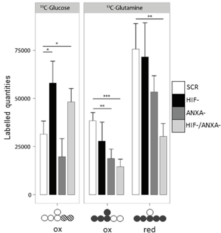
Figure 5: Reductive carboxylation is reduced in HIF-/ANXA- AGS cells. (A) Schematic representation of the different mass isotopomers of citrate and the corresponding origin via the different labelling substrates U-^{13}C_6 -glucose and U-^{13}C_5 -glutamine. Three different mass isotopomers of citrate are the result of oxidative (ox) and reductive (red) carboxylation (○○○●, ●●●○○ and ●●●●●). (B) Shown are the corresponding labelled quantities of the detectable C5-fragment of citrate ( n = 3 ; mean \pm SD; * P < 0.05 ; ** P < 0.01 ; *** P < 0.001 ) for control (scr) and the different knock-down AGS cells.
