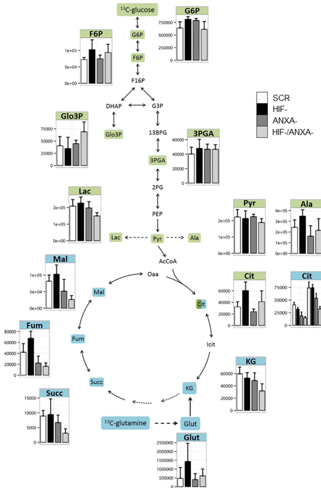
Figure 3: Activity of the central carbon metabolism of AGS cells estimated by pSIRM. Glycolytic and TCA cycle activity of the different AGS knock-down derivatives was determined by 13 C-glucose (green) and 13 C-glutamine (blue) pSIRM experiments ( n = 3). Labelled quantities of the different intermediate metabolites are shown. Abbreviations: 13BG: 1, 3 bis-phosphoglycerate; 2PG: 2-phosphoglycerate; 3PG: 3-phosphoglycerate; AcCoA: acetyl coenzyme A; Ala: Alanine; Cit: citrate; DHAP: dihydroxyacetone-phosphate; F6P: fructose 6-phosphate; F16P: fructose 1, 6 bis-phosphate; Fum: fumarate; G3P: glyceraldehyde-3-phosphate; G6P: glucose 6-phosphate; Glut: glutamate; Icit: iso-citrate; KG: alpha-ketoglutarate; Lac: lactate; Mal: malate; Oaa: oxaloacetate; PEP: phosphoenolpyruvate; Pyr: pyruvate; Succ: succinate.
