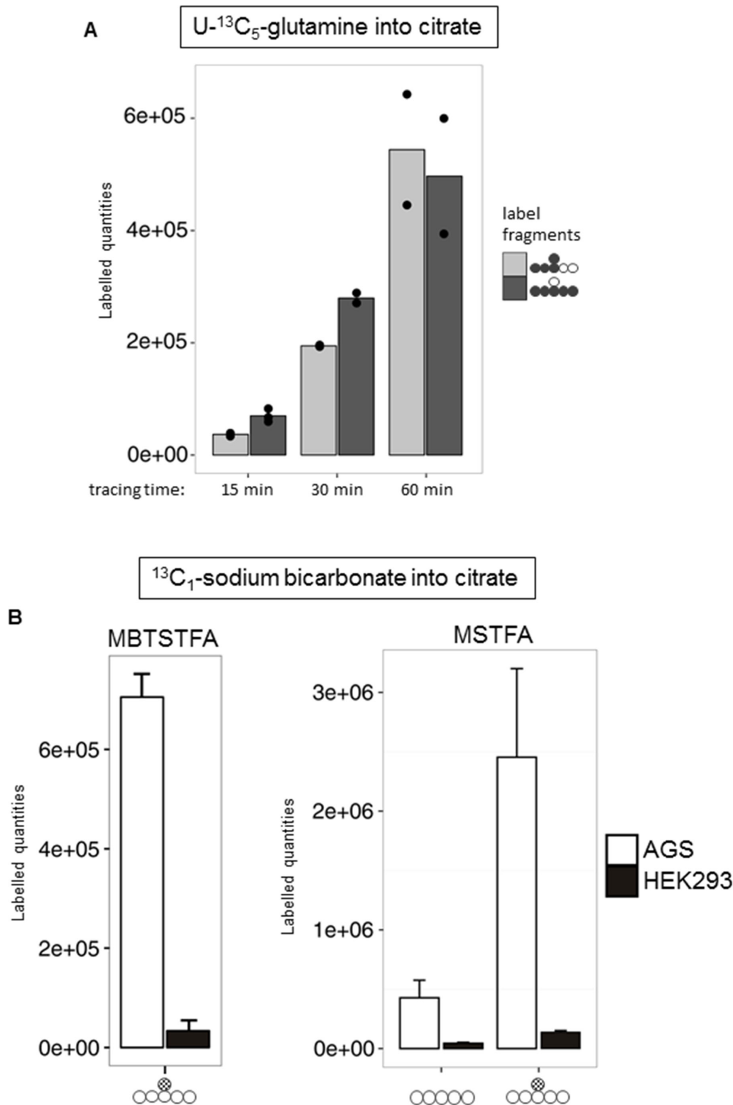
Figure 4: Evidence for reductive TCA metabolism via 13 C 5 -glutamine and 13 C 1 -HCO 3 labelling. (A) Time series pSIRM analysis of AGS wild type cells with U- 13 C 5 -glutamine for 15, 30 and 60 min ( n = 3 , n = 2 and n = 2 , respectively) under normoxic conditions. Labelled quantities for citrate (looking at m + 3 and m + 5 mass shift of the C5 fragment; for easier recognition full metabolite is depicted by circles) at these three time points are shown (mean \pm SD, n = 3 ). (B) Comparison of the derivatization agents MBTSTFA and MSTFA for citrate detection. Left (MBTSTFA): AGS wild type and HEK293 cells were labelled with 13 C 1 -sodium bicarbonate for 20 min under normoxic conditions. Carbon fixation was observed by a mass shift on m + 1 of citrate ( m/z = 459 ). Right (MSTFA): Same labelling conditions, measurement in splitless mode for improved detection of the C6-fragment. Depicted is the C5-fragment ( m/z = 273 ) compared to the m + 1 of the C6-fragment ( m/z = 375 ) of citrate. Values are means \pm SD of three independent experiments.
