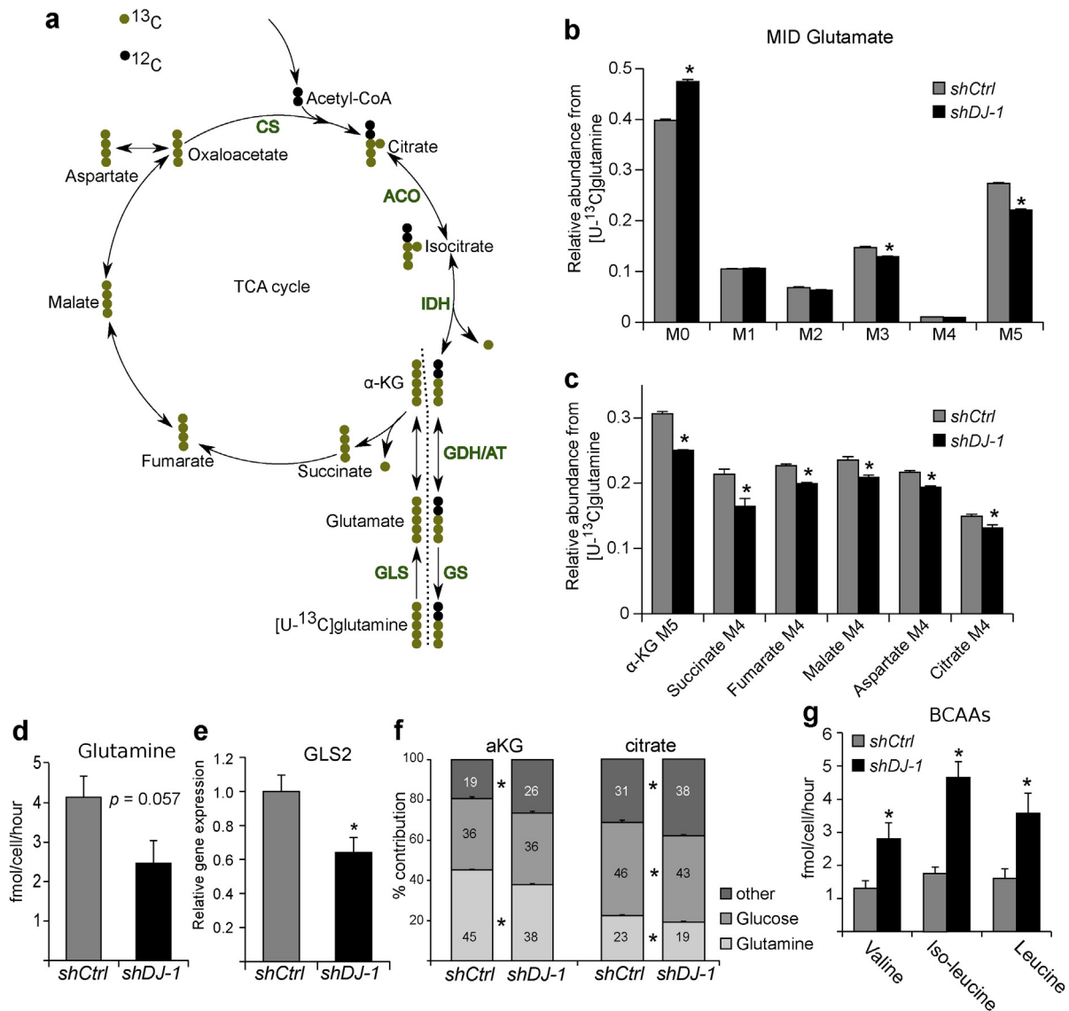
Fig. 4. Metabolic profiling of DJ-1 silenced LUHMES cells reveals decreased glutamine influx. (a) Schematic of atom transitions in central metabolism using [\text{U-}^{13}\text{C}]\text{glutamine} as a tracer. ^{13}\text{C} carbons are in green, ^{12}\text{C} in black. ACO: aconitase; AT: aminotransferase; CS: citrate synthase; GDH: glutamate dehydrogenase; GLS: glutaminase; GS: glutamine synthetase; IDH: isocitrate dehydrogenase. The dotted line indicates beginning and end of one cycle. (b–c) Application of [\text{U-}^{13}\text{C}]\text{glutamine} as a tracer in LUHMES cells for determination of MID to infer relative intracellular fluxes. (b) MID of glutamate. (c) Relative abundance of M5 aKG, M4 succinate, M4 fumarate, M4 malate, M4 aspartate and M4 citrate. (d) Glutamine consumption from the medium. (e) Gene expression of GLS2 . (f) Carbon contribution of glucose, glutamine and other carbon sources (%) to aKG and citrate. (g) Branched chain amino acid consumption. Error bars represent SEM. Asterisks indicate a significant difference to the respective shCtrl . (Welch's t-test, p < 0.05 ; number of biological replicates: n \geq 3 ). See also Supplementary Fig. S4.
