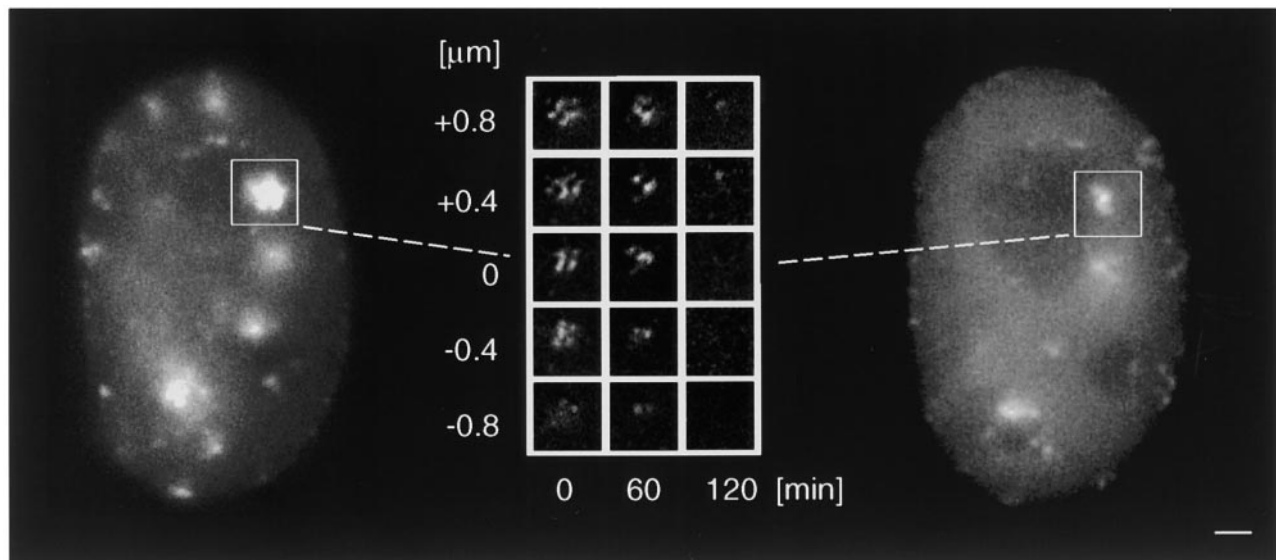
Figure 5. Larger replication foci are composed of independent smaller foci. One late S phase nucleus of a stably transfected cell was imaged over 2 h. Together with small size foci (less than 1- \mu\text{m} diam) several large foci are visible at the beginning of the experiment (left side nucleus). 2 h later some new small foci have formed and the large ones did not change their nuclear position, but decreased in size concomitantly with an increase in the disperse nucleoplasmic GFP-PCNAL2 protein (right side nucleus). Deconvolved images from different Z planes (middle) reveal that these large foci are made of clusters of small size foci which form and disassemble independently giving rise to the different shapes and sizes of the large foci over time. The signal (within the white box) seen in the undeconvolved whole nucleus after 2 h (right image) comes from out-of-focus light from the planes above. Bar, 1.5 \mu\text{m} .
